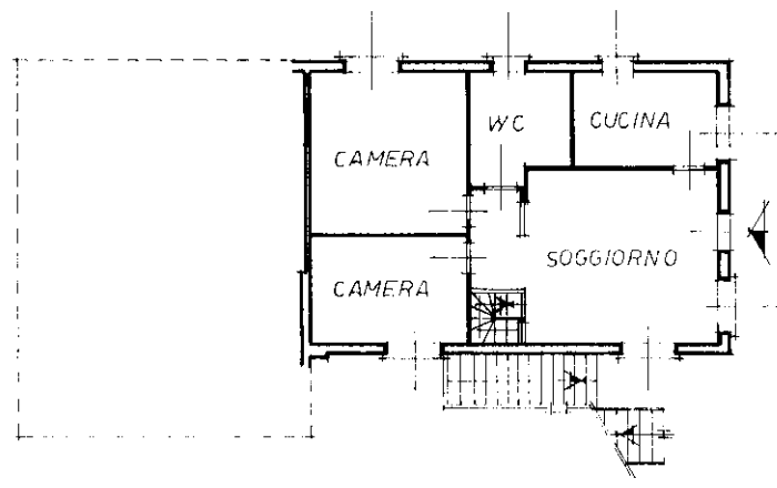
PIANO TERRENO H=255
